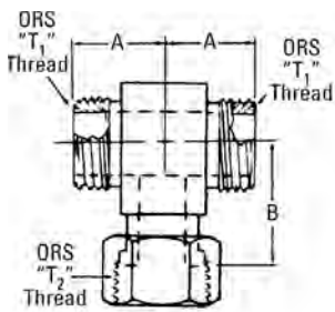
FF1857T(Dash size) (Ref. SAE 520433) (Formerly Weatherhead Series 4707x)
